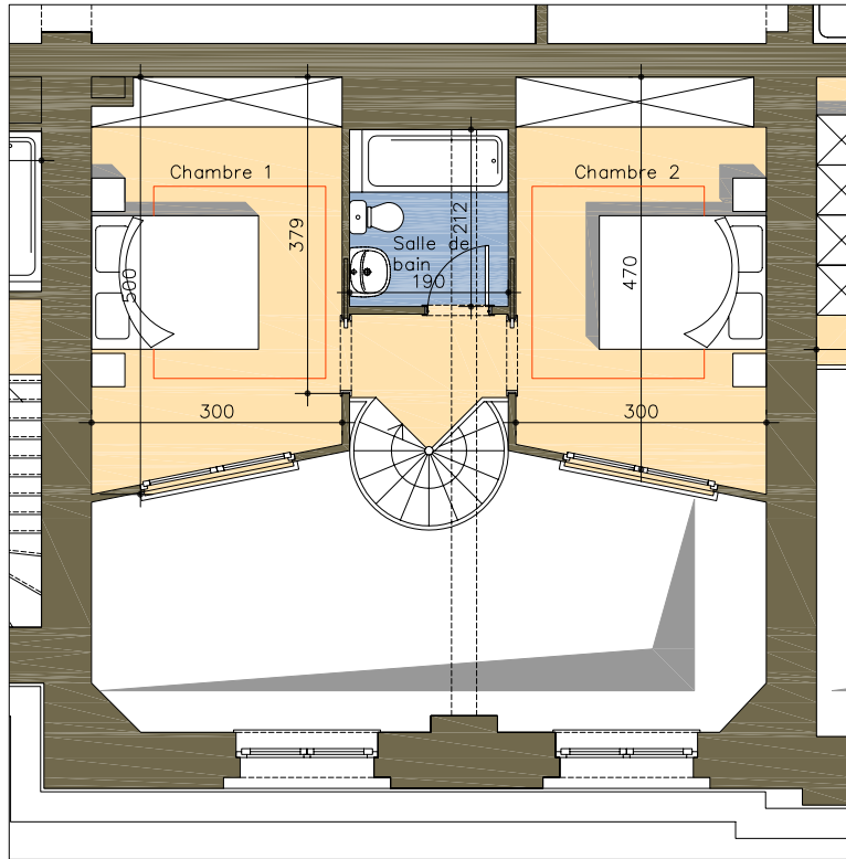
Mezzanine
